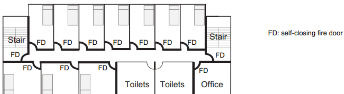
Figure 4 Protected bedroom corridor
