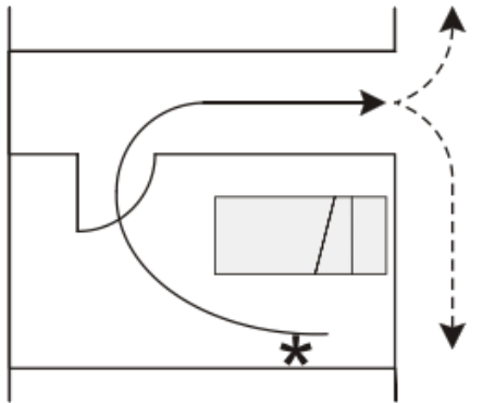
Figure 7 – Single Direction of Escape Out of Room and Along a Corridor Before a Choice of Escape Routes Become Available
