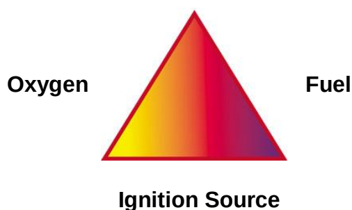
Figure 2 Triangle of fire
