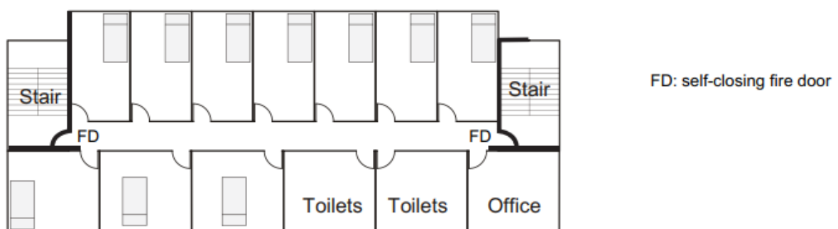
Figure 10 - Protection of Escape Stairs
