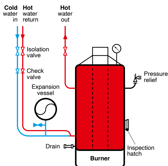
Figure 2.7 Direct-fired (gas) water heaters
